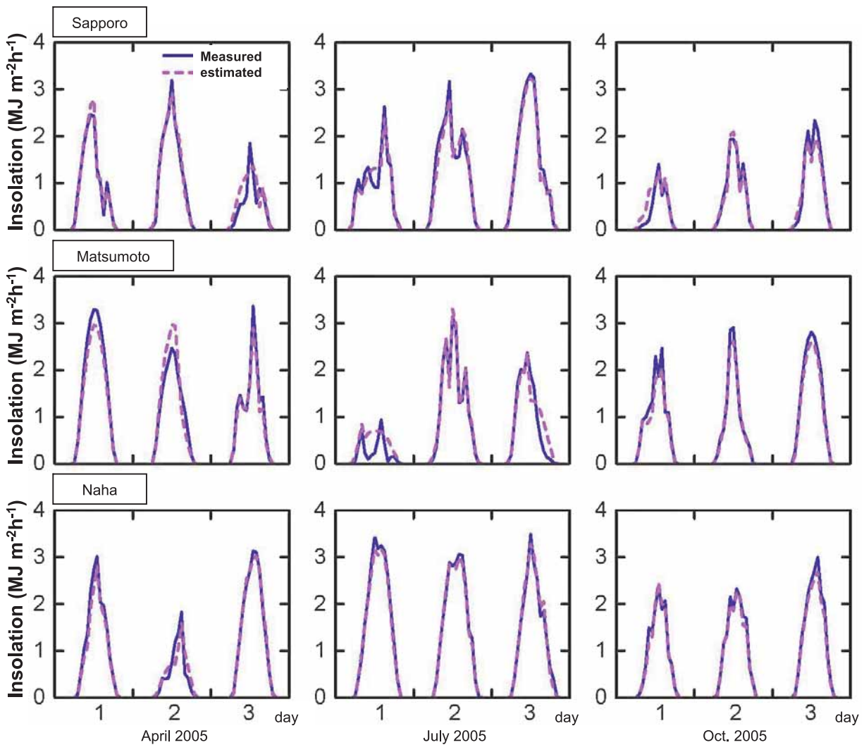
Fig. 4 Comparison of estimated and measured insolation in Sapporo, Matsumoto, and Naha
