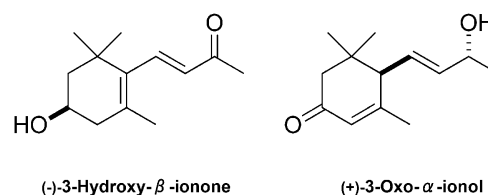
Fig. 1 Structural formulae of (–)-3-hydroxy-β-ionone and (+)-3-oxo-α-ionol
