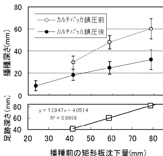
図2-47 播種床の矩形板沈下量と播種深さ
